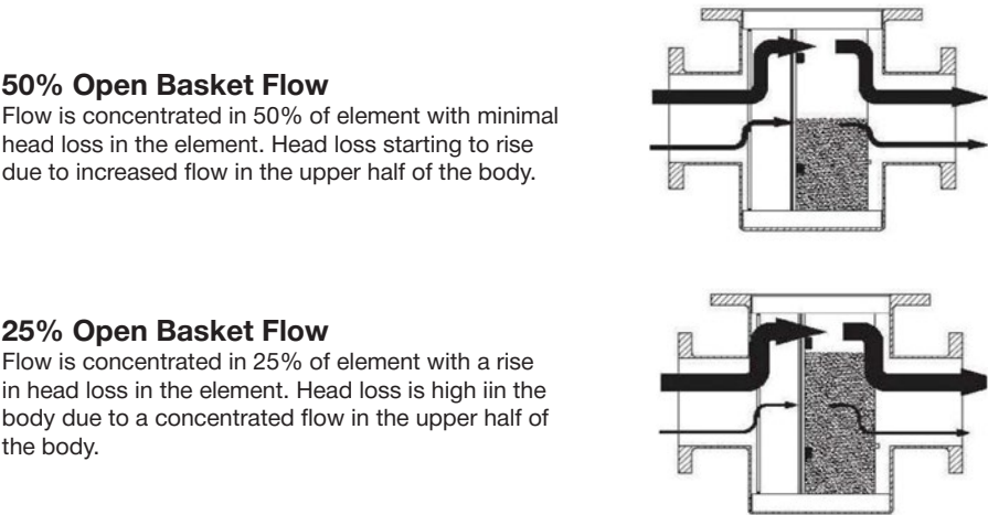
FIGURE 2 - FURTHER SOLIDS COLLECTION UP TO THE SCREENING PHASE
