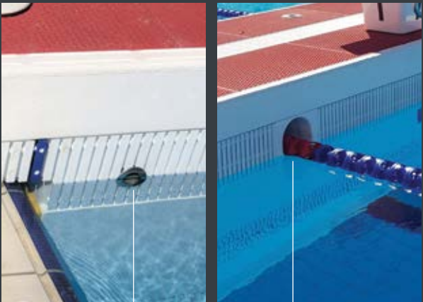
Fixed 316 stainless steel cup anchors for outside lanes
